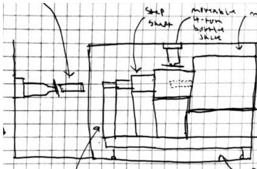
Figure 7: Stepped Bearings
