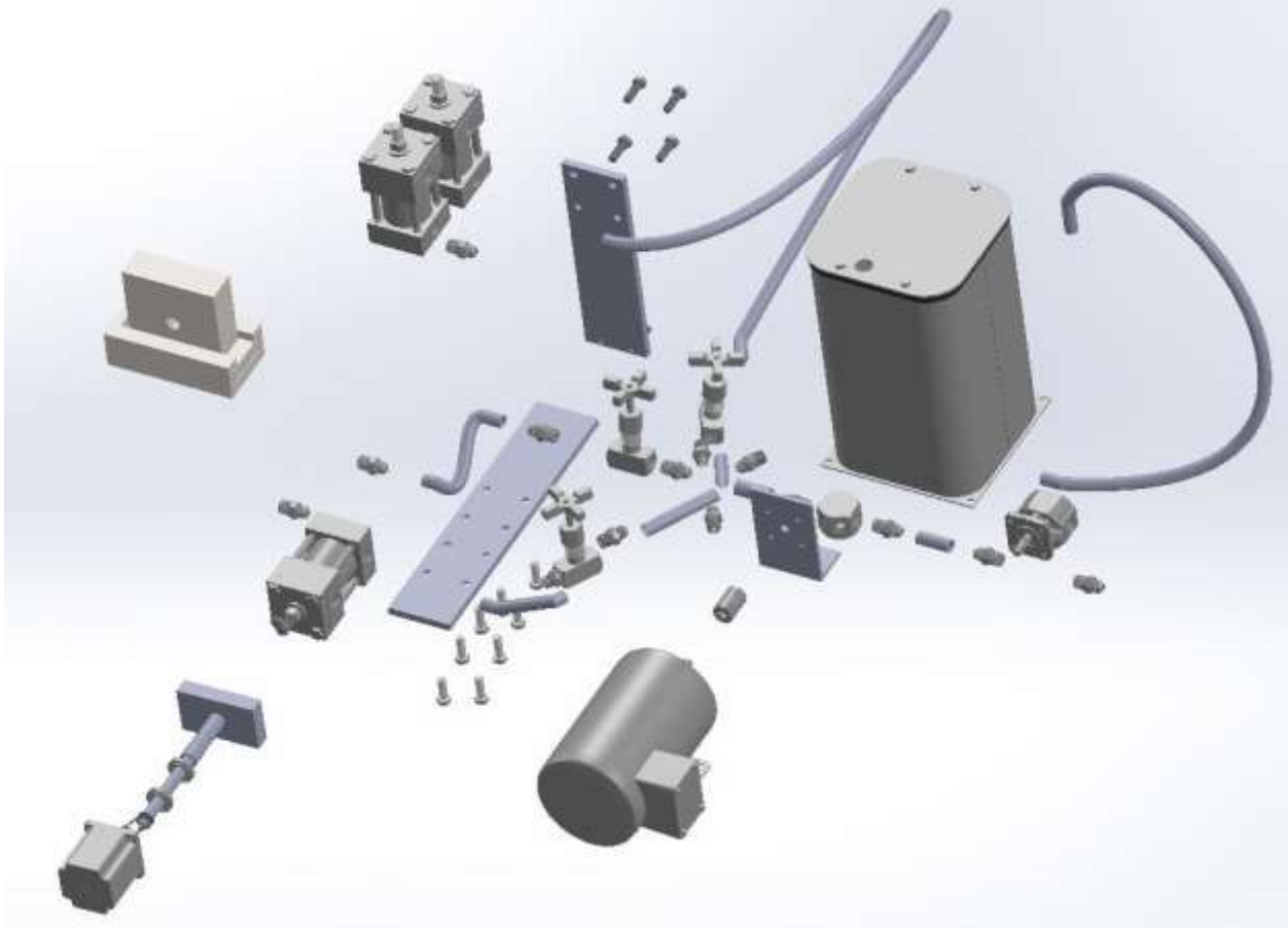
Figure. 11 Exploded view of CAD model
