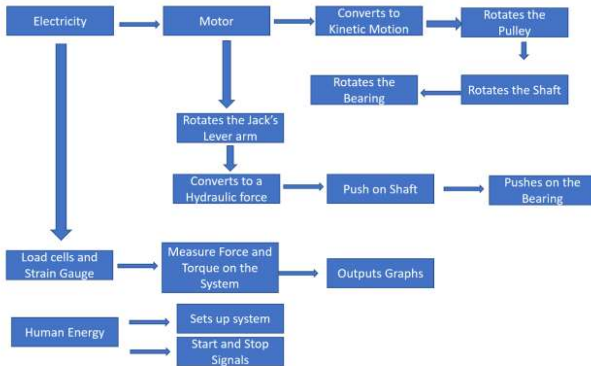
Figure 4: Functional Model
