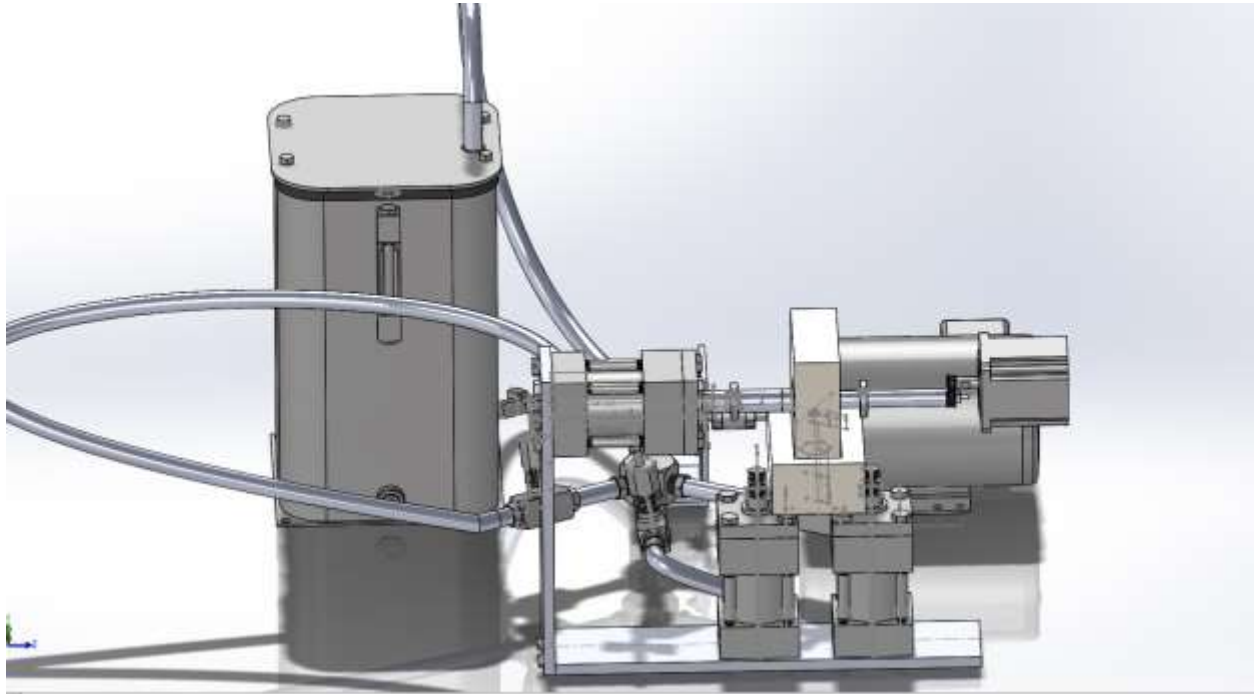
Figure 10: Solidworks Model of Design
