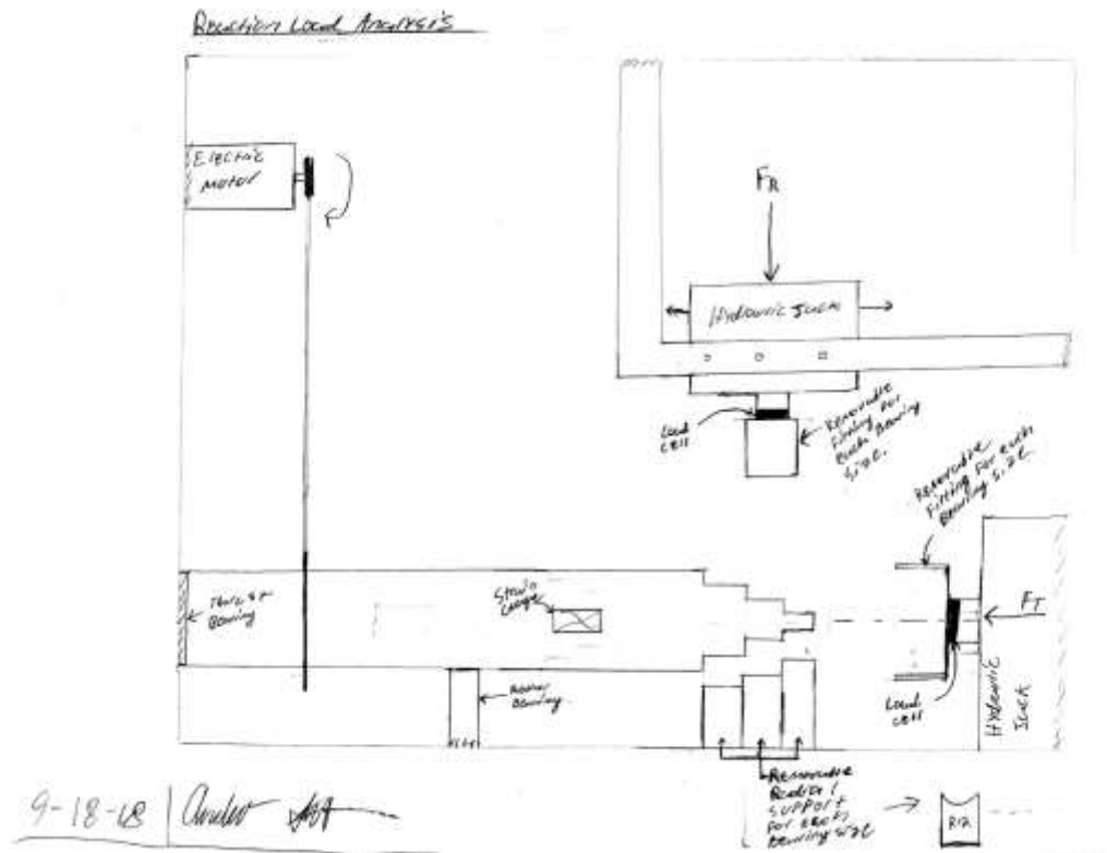
Figure 9: Reaction Load Analysis
